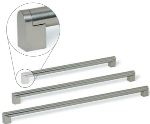
OD22 Steel Bar Handles. Ref 331: 160mm centre/188mm overall Ref 332: 309mm centre/337mm overall Ref 333: 627mm centre/655mm overall
